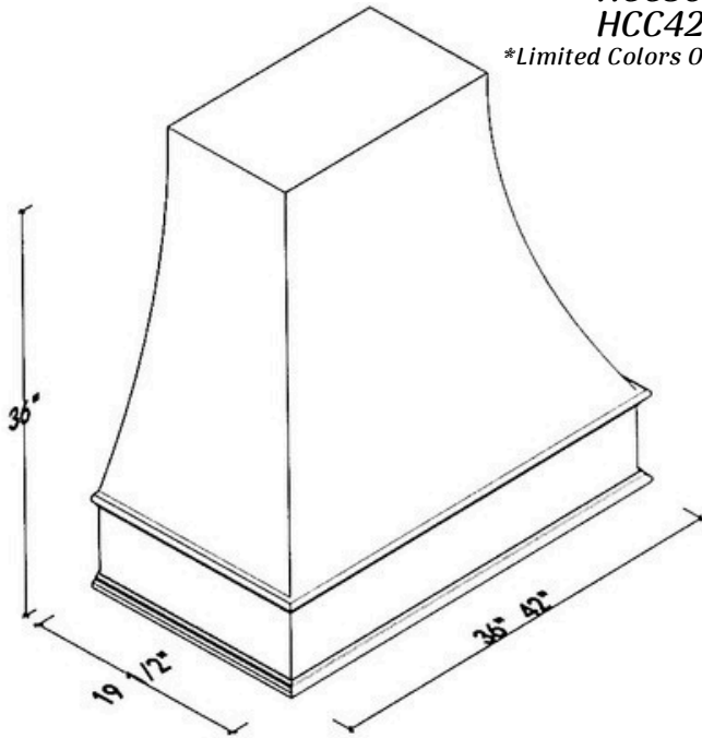
Decorative Hood Cover
